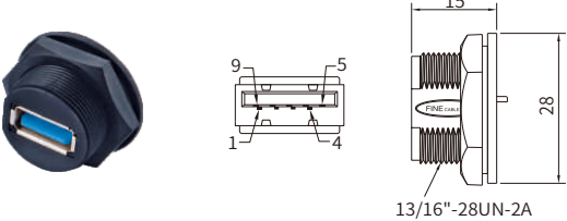
USB3.0
